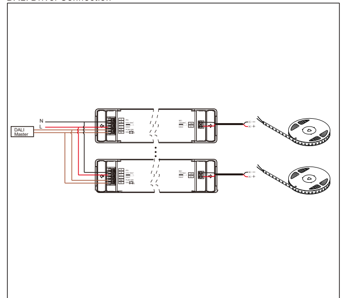
DALI Driver Connection
