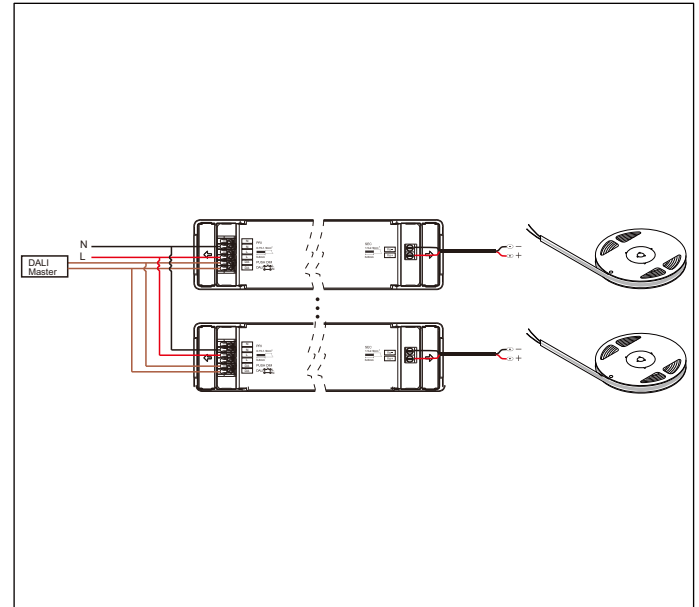
DALI Driver Connection
