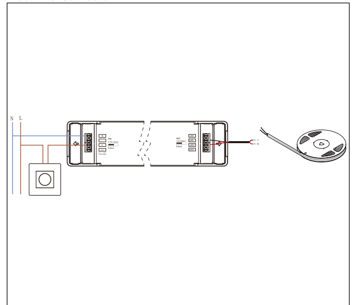
Triac Driver Connection
