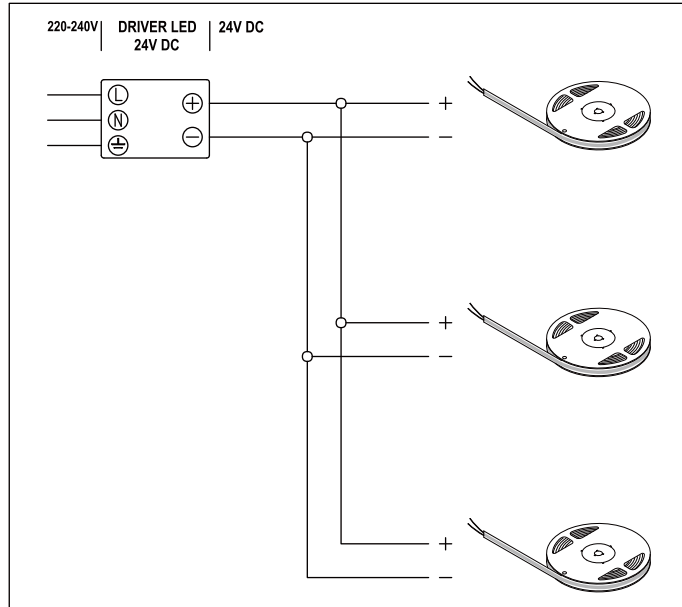
ON/OFF Connection
