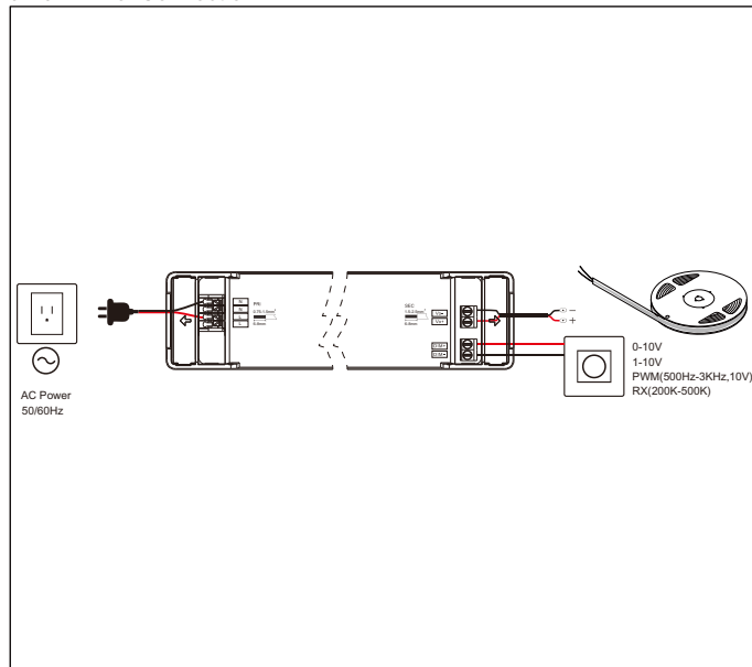
0-10V Driver Connection
